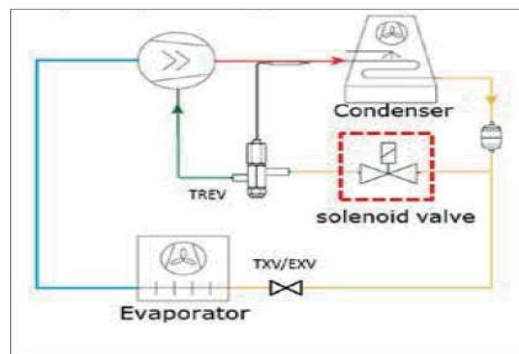
Liquid injection system configuration
